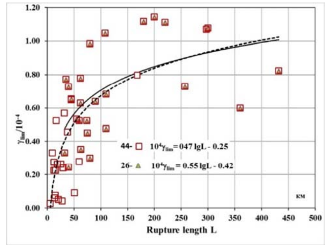
Figure 6b. Dependence between of \gamma_{lim} rupture length L (km).
