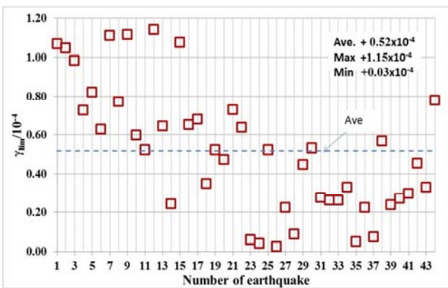
Figure 4a. Distribution of \gamma_{lim} ultimate deformations values a- for 44 earthquakes with 5.6≤M≤8.5.
