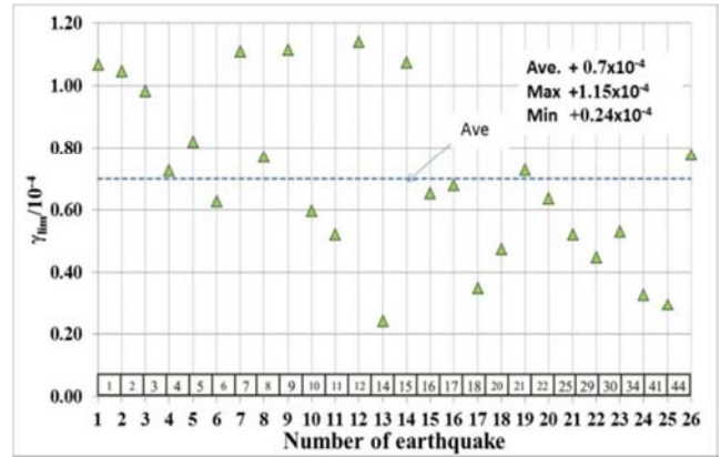
Figure 4b. Distribution of \gamma_{lim} ultimate deformations values b- for 26 earthquakes with M≥7.0.
