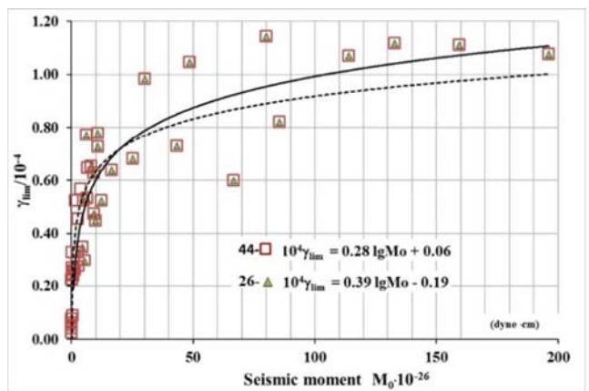
Figure 6c. Dependence between of \gamma_{lim} (m) and seismic moment M_0 .
