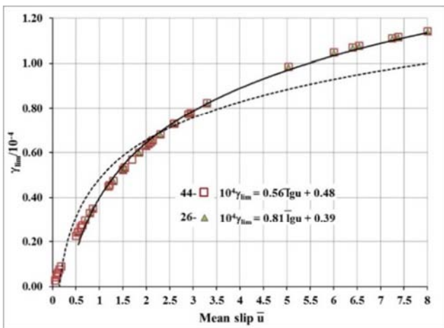
Figure 6a. Dependence between of \gamma_{lim} and average slip \bar{u} (m) length.
