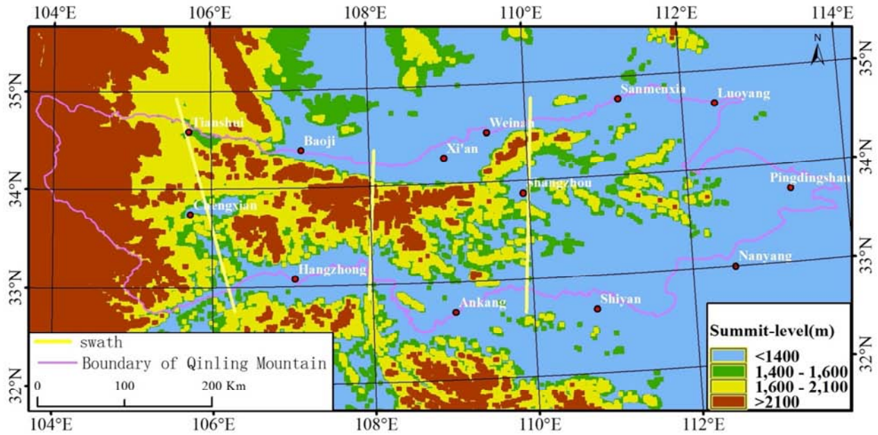
Fig. 3. The summit-level map of Qinling Mountain.
