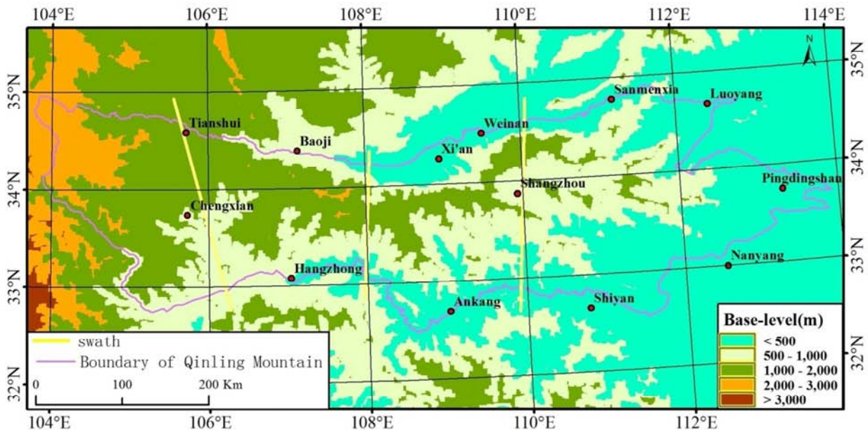
Fig. 4. The Base-level map of Qinling Mountain.
