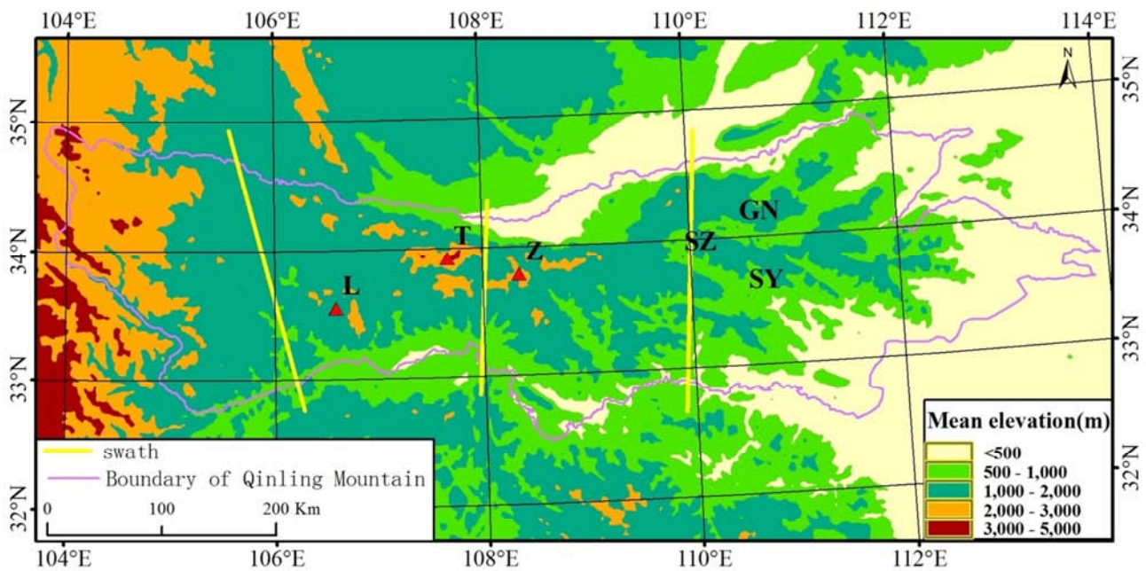
L: Liuba Mountain, T: Taibai Mountain, Z: Zhongnan Mountain, SZ: Shangzhou Basin, SY: Shangyang Basin, GN: Genan Basin
