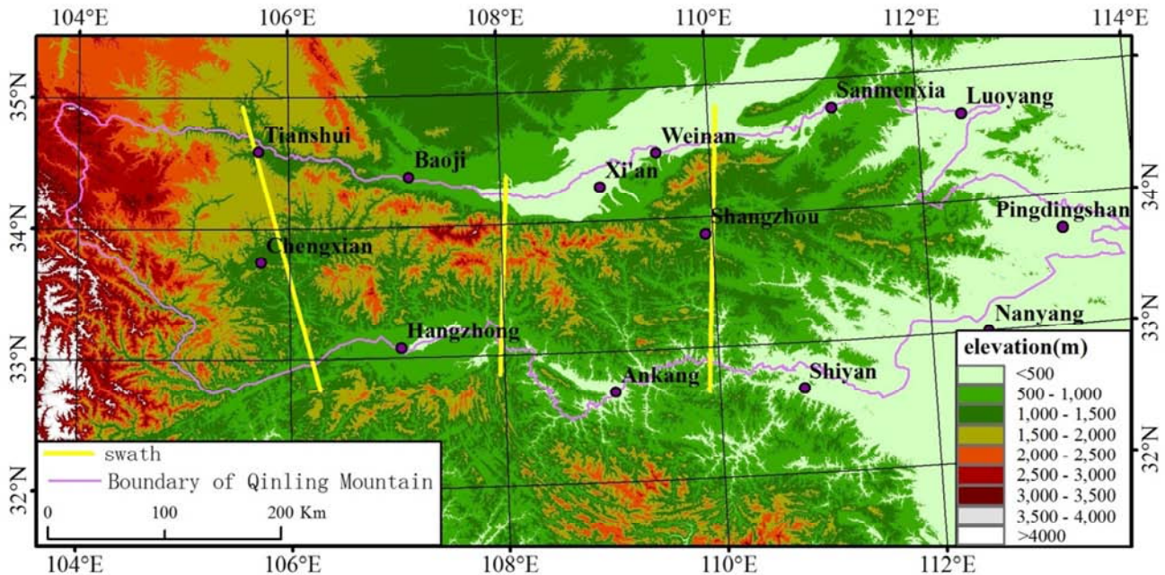
Fig. 1. The DEM of Qinling Mountain.
